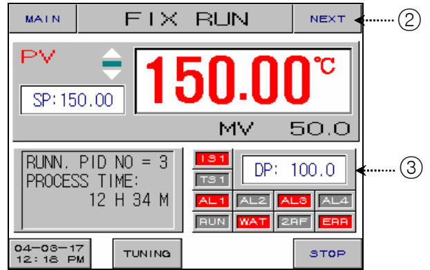
Figure 2-24. Fix Run- 3 screen
