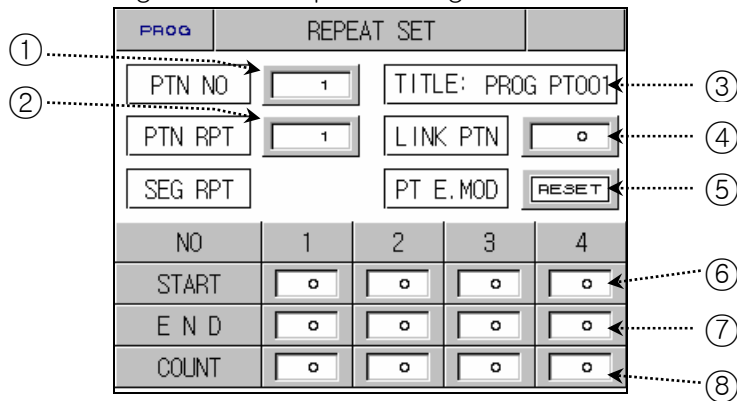
Figure 2-41. Repeat Setting Screen
