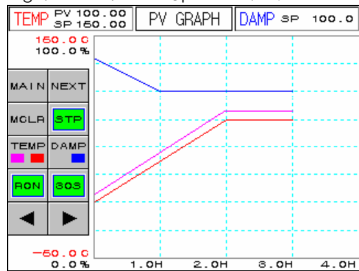
Figure 2-20. Fix Stop - 2 screen
